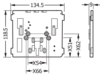
Size 1 wall mounting
