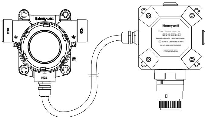
XCD RTD with Remotely installed sensor
